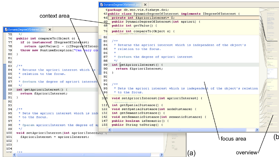
Figure 8: Fisheye Java sourcecode browser, based on the ideas from the Furnas Fisheye. Image from [33] © 2006 ACM, Inc. Reprinted by permission.
