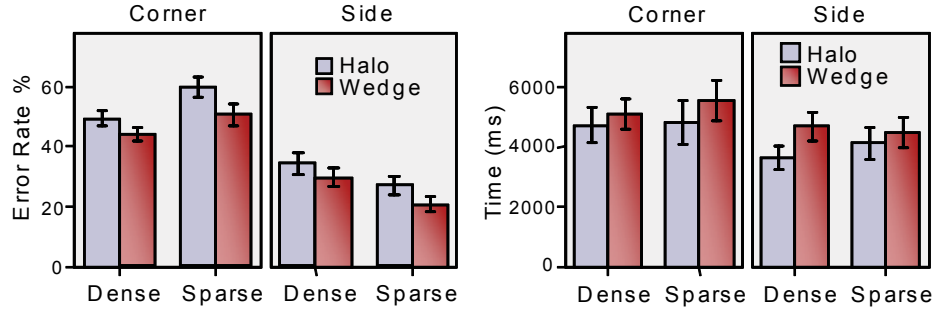
Figure 28: Closest task error amount and completion times by visualization, density, and position. Error bars indicate \pm 1 standard error.
